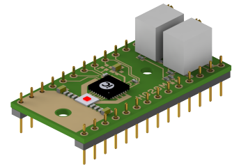
Figure 1: HG20M Package (DIL28)
